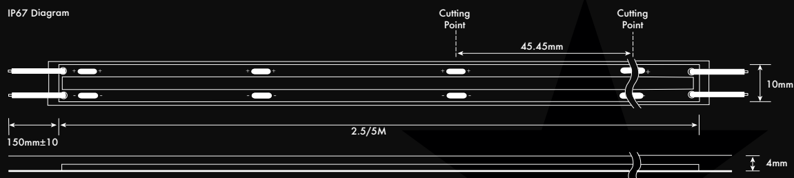
IP67 Diagram
