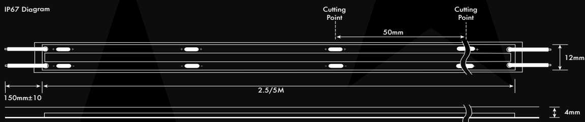
IP67 Diagram
